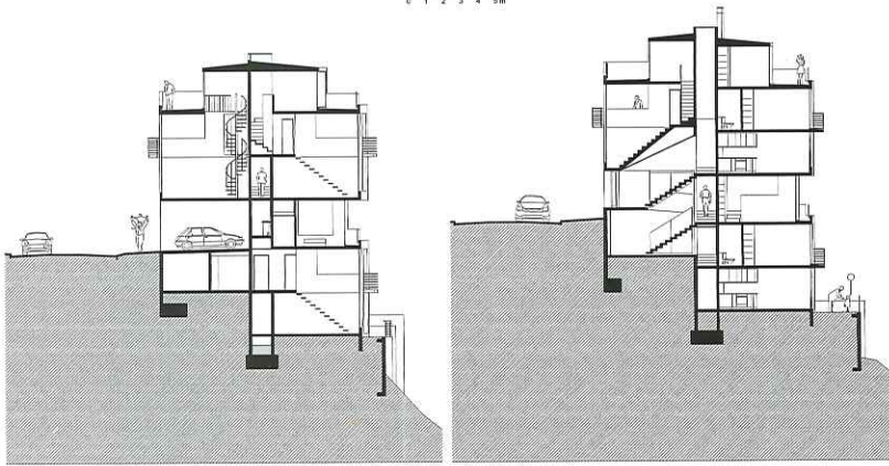
CROSS SECTION B
